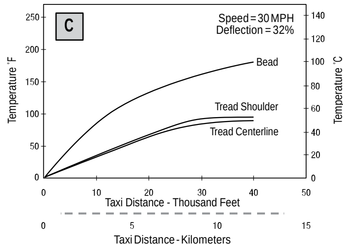
Temperature Rise vs Taxi Distance
