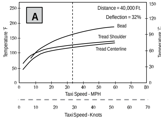
Temperature Rise vs Taxi Speed
