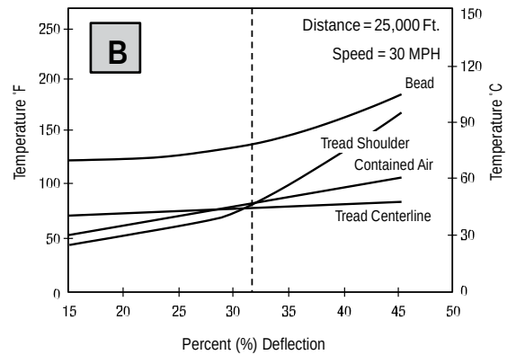
Temperature Rise vs Percent Deflection
