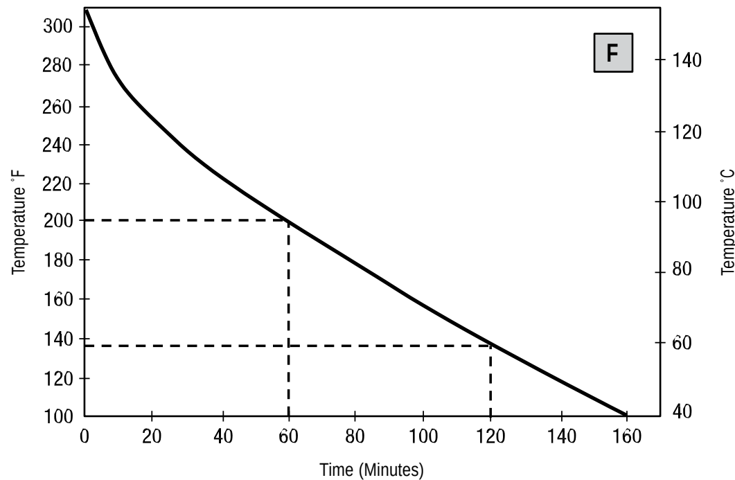
Time for Tire Temperature to Dissipate
